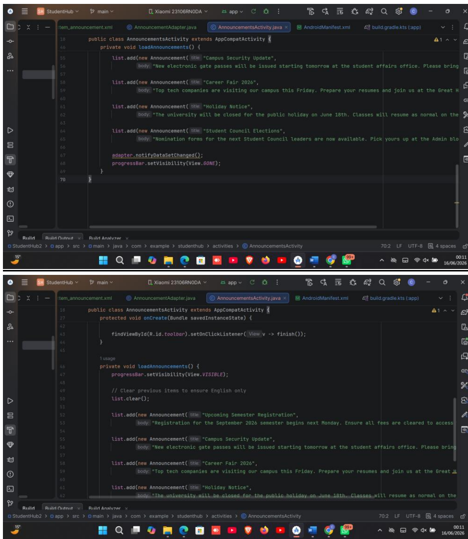
Figure 28ANNOUNCEMENT JAVA CODE
