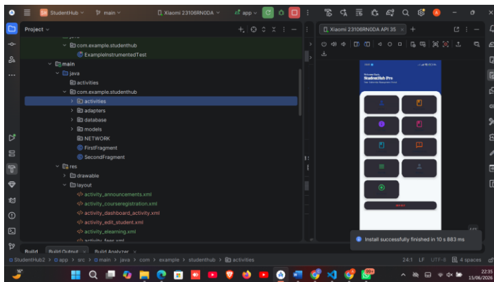
Figure 16 ANDROID STUDIO
